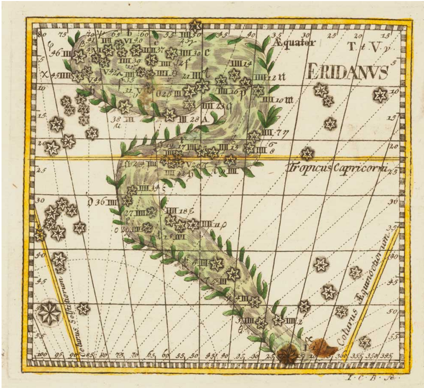
18th century illustration of the Eridanus constellation
