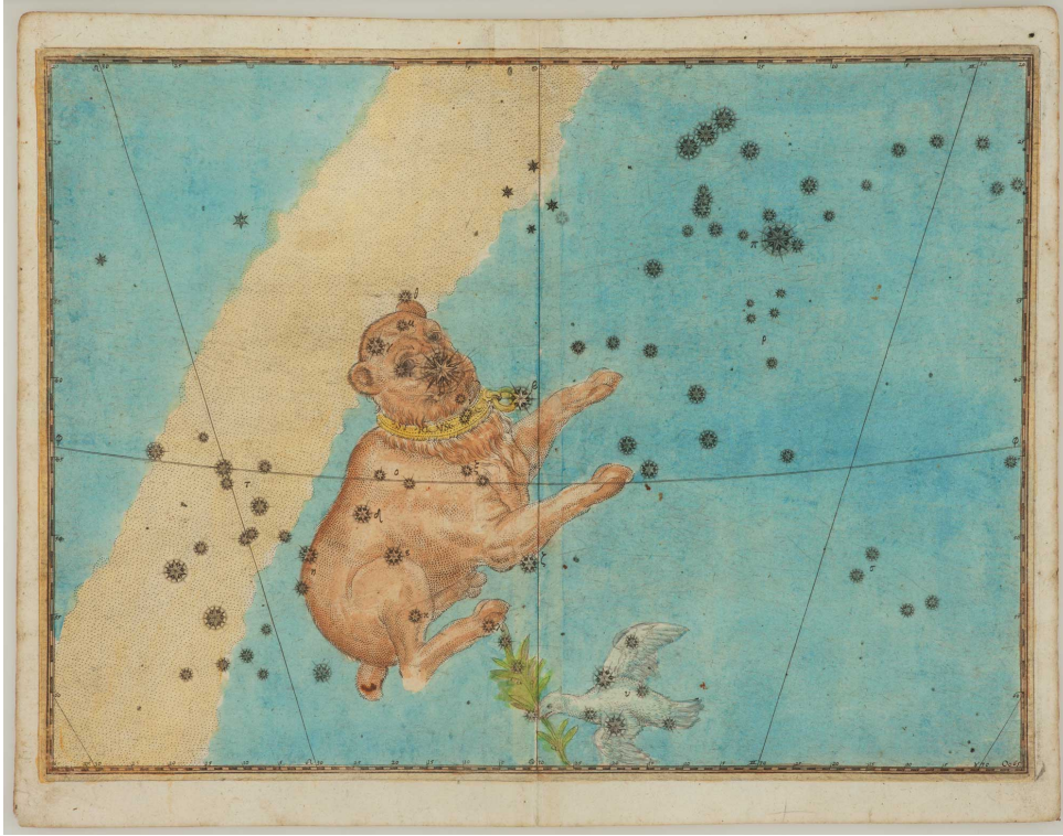
A 17th century illustration of the constellation of Canis Major
