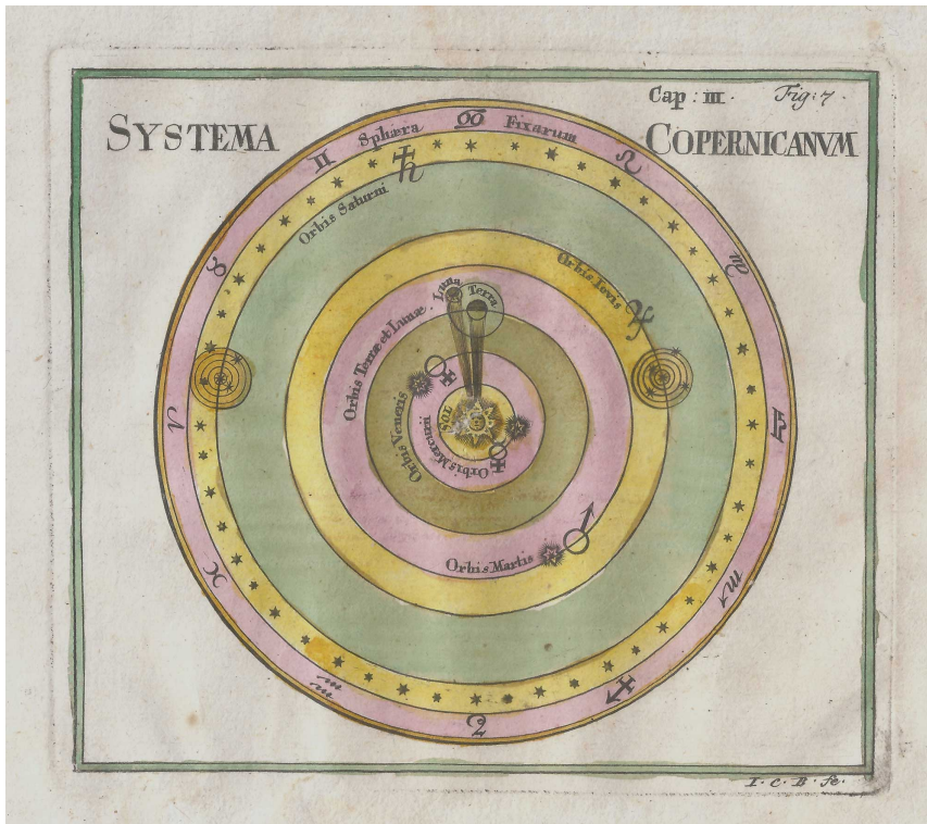
18th century illustration of the Copernican Solar System
