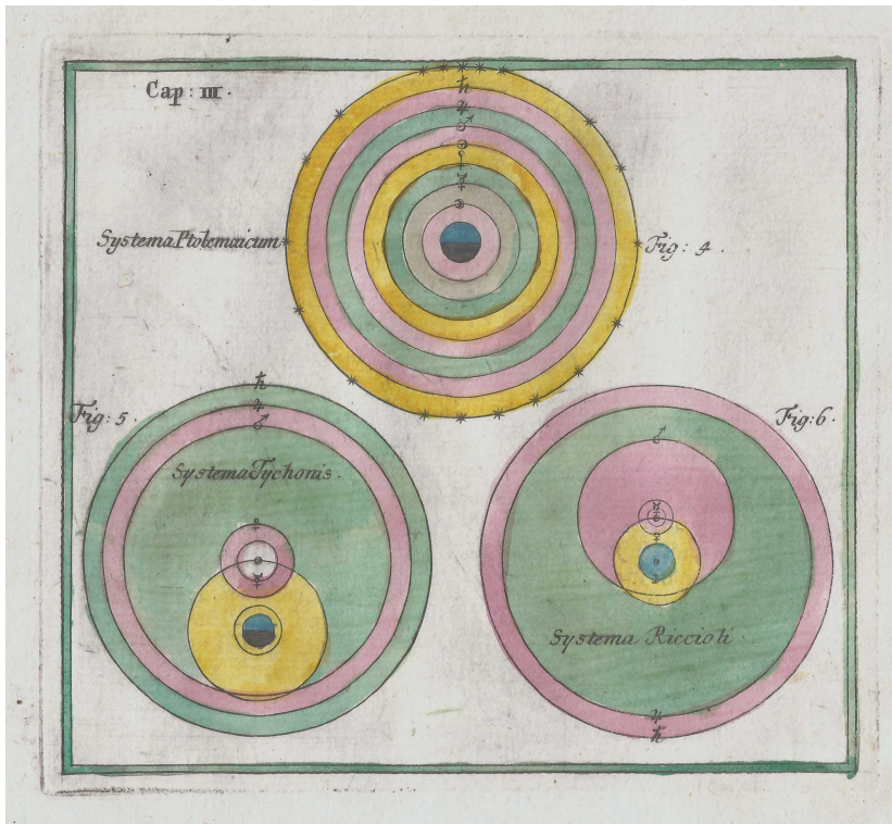
The Solar Systems according to Ptolemy, Brahe and Riccioli
