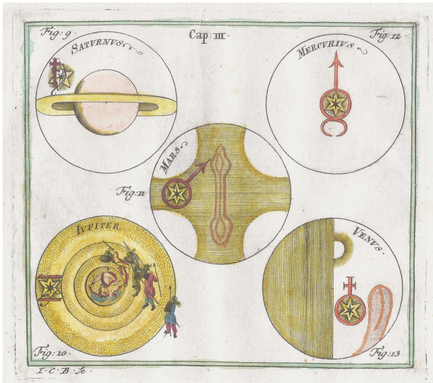
18th century illustration of the known planets
