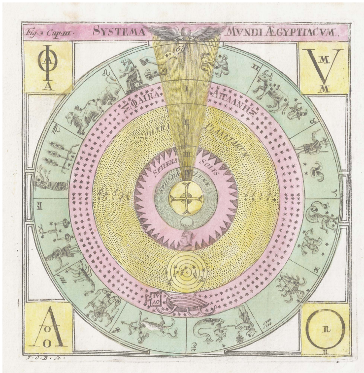
18th century illustration of the Solar System of the Ancient Egyptians
