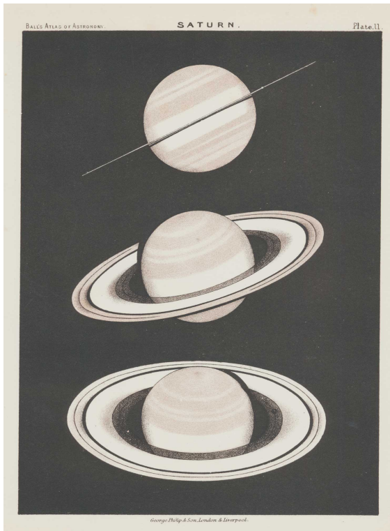
19th century chart of Saturn
